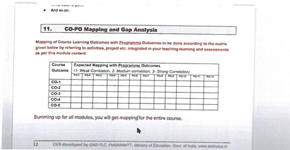
Photo 24: CO/PO mapping
